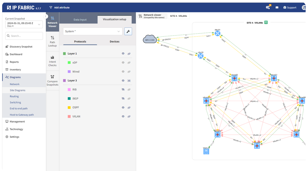
The visualization flexibility of an automatically generated network topology map
