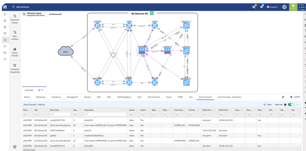
Firewall Policy Implementation as Visualized in IP Fabric
